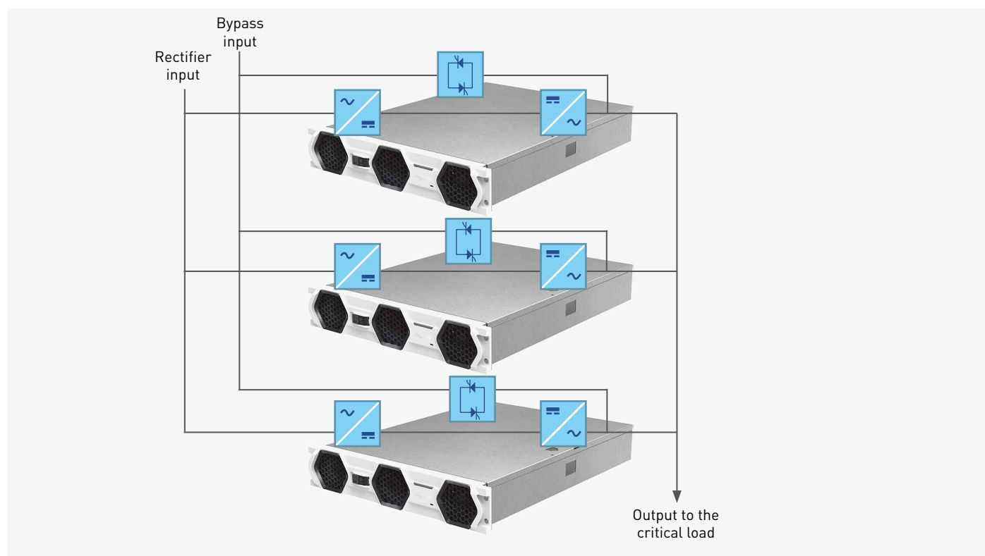
Figure 4: Modular UPS with N+X Redundancy
