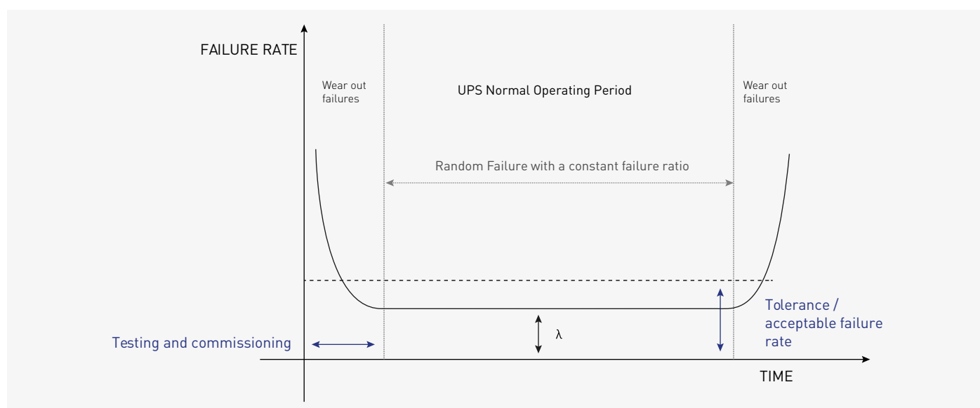
Figure 1: Failure rate ( \lambda ) as function of the time
