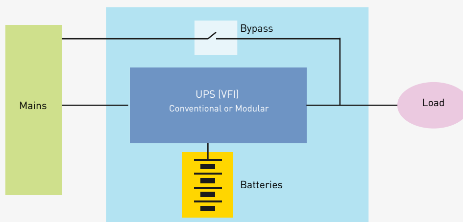
Figure 2: Schematic Block Diagram of UPS system
